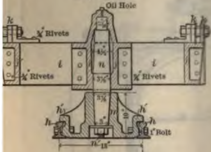
SECTION A B. REVOLVED TO SIDE.
